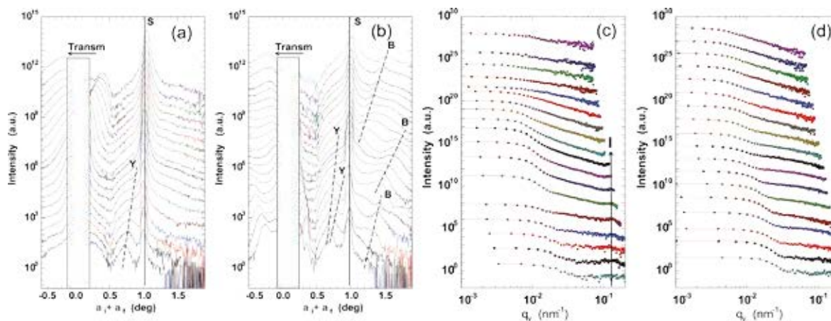
Figure 2: (a) and (b), vertical line cuts of the 2D data as a function of the detector angle ( \alpha_1 + \alpha_2 ) for 60 nm and 300 nm film thickness, respectively. The position of the specular peak (S) is indicated by the solid line. The position of the Yoneda peak (Y) and Bragg peak (B) are indicated by the dash line, respectively. (c) and (d), horizontal line cuts of the 2D data as a function of the q_y for 60 nm and 300 nm film thickness.
