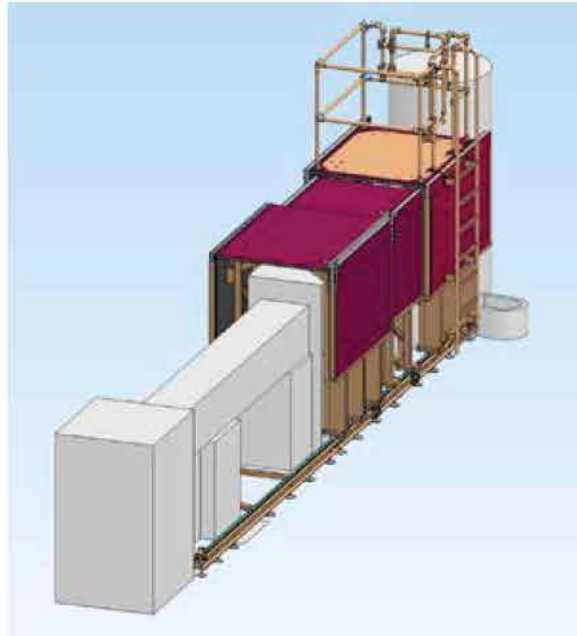
Figure 10: New shielding design implemented at RESEDA.
