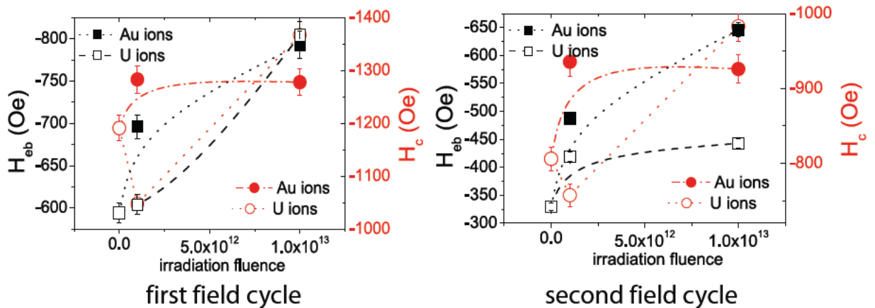
Figure 1: Plots of H_{\text{eb}} (squares) and H_c (circles) as a function of irradiation fluence of Au and U ions respectively during the first and second hysteresis field cycles after field cooling to 10 K.
