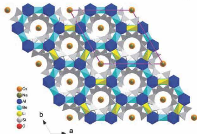
Figure 1: The crystal structure of pezzottaite viewed down [0001] .
