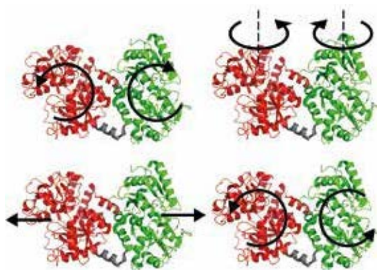
Figure 4: Motion patterns of the dominant normal modes 7–10.
