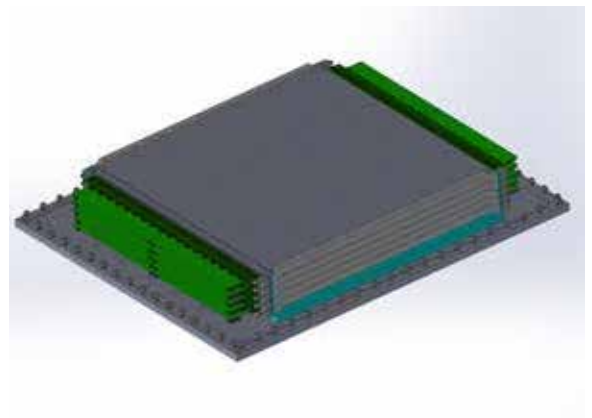
Figure 4: Design study of a 40 x 40 cm 2 detector with solid Boron converter with macro-structured topology developed at FRM II.
