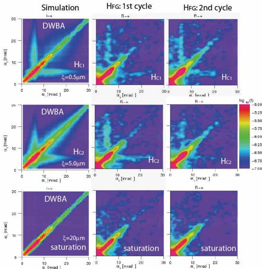
Figure 1: SF intensity maps from representative IrMn/CoFe samples for the field growth condition and measured at the coercive fields HC1 (along the first half of the first field cycle - untrained), HC2 (along the second half of the first field cycle) and that at saturation. The measurements for the second field cycle (trained) are also shown alongside with DWBA simulated patterns. Here \alpha_{i,t} are the incident and exit angles.
