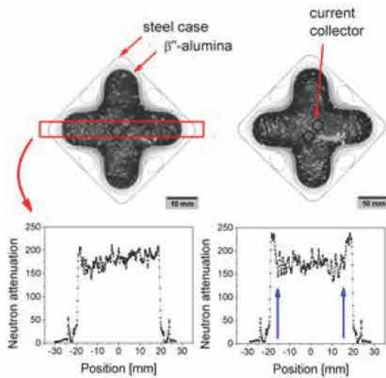
Figure 2: Horizontal reconstructed slices of the discharged (left) and the half-charged battery cell (right) from the tomography measurements at ANTARES. The red rectangle identifies the section of the slices from which the line profiles (below) were extracted.
