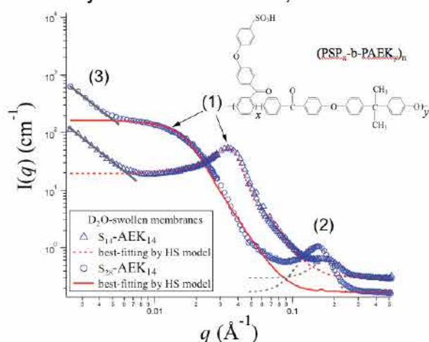
Figure 1: Molecular structure of (PSP_x-b-PAEK_y)_n and SANS profiles for D_2O -swollen membranes.
