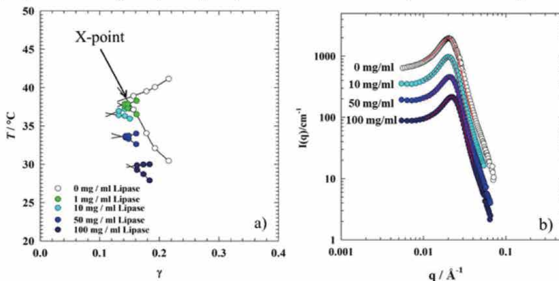
Figure 1a): Phase diagrams of microemulsions of type H_2O/NaCl (4 wt%) – n-octane – C_{10}E_6 – CAL B. The X-points run through a maximum in efficiency, the phase boundaries continuously shift to lower temperatures. b) SANS curves of the base microemulsion and a CAL B concentration series. The characteristic structure peaks were fitted to the Teubner-Strey model.
