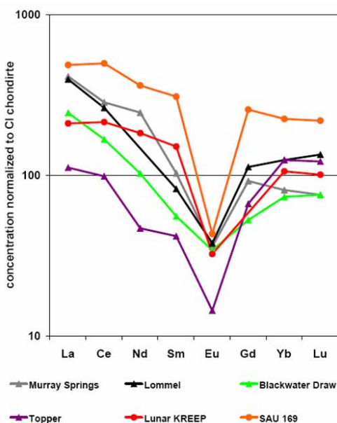
Figure 2: PGAA/NAA analysis of the YD layer at many sites shows negative Eu anomalies observed only in lunar KREEP and in SAU 169, a meteor from Oman, believed to have originated from the Procellarum Lunar KREEP Terrane region of the moon.
