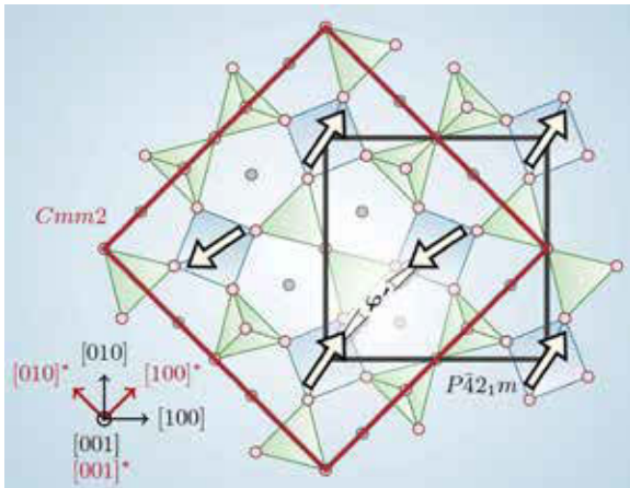
Figure 1: Magnetic structure of BCGO at 2.2 K: View along the [001] direction. Both P-42_1m and Cmm2 crystallographic unit cells are shown.
