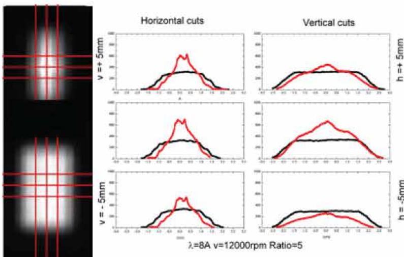
Figure 14: Left: Beam cross section, at \lambda = 8 \text{ \AA} , measured with a detector at the sample position - focusing guide (top) vs. linear guide (bottom); Right: Horizontal and vertical beam profile. Horizontal and vertical cuts taken at the centre of the beam and around 1 \text{ cm}^2 area centred around it - focusing guide (red) vs. linear guide (black).
