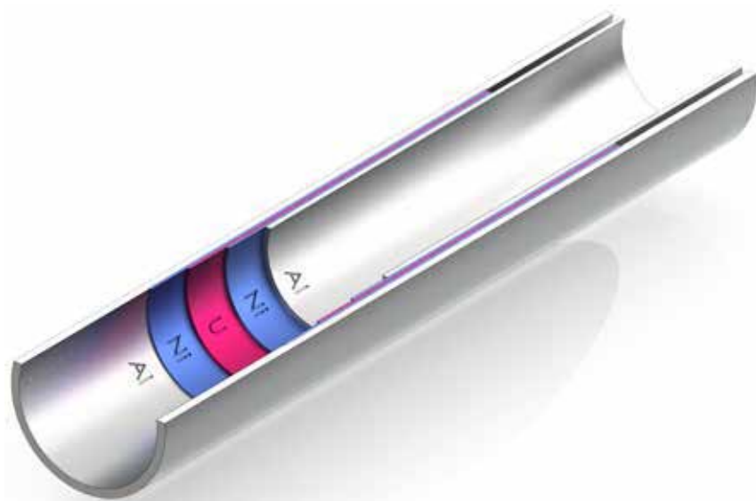
Figure 1. Sectional drawing of a cylindrical Mo-99 target.
