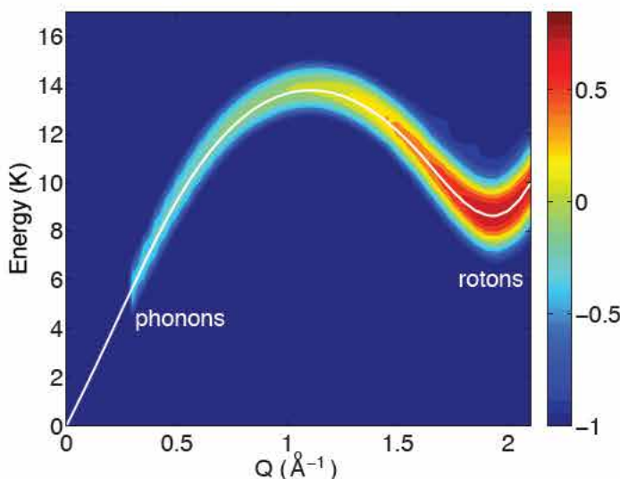
Figure 1: Phonon-rotor dispersion in superfluid ^4\text{He} . The color coding corresponds to the logarithm of the intensity of neutrons scattered from the quasiparticles.
