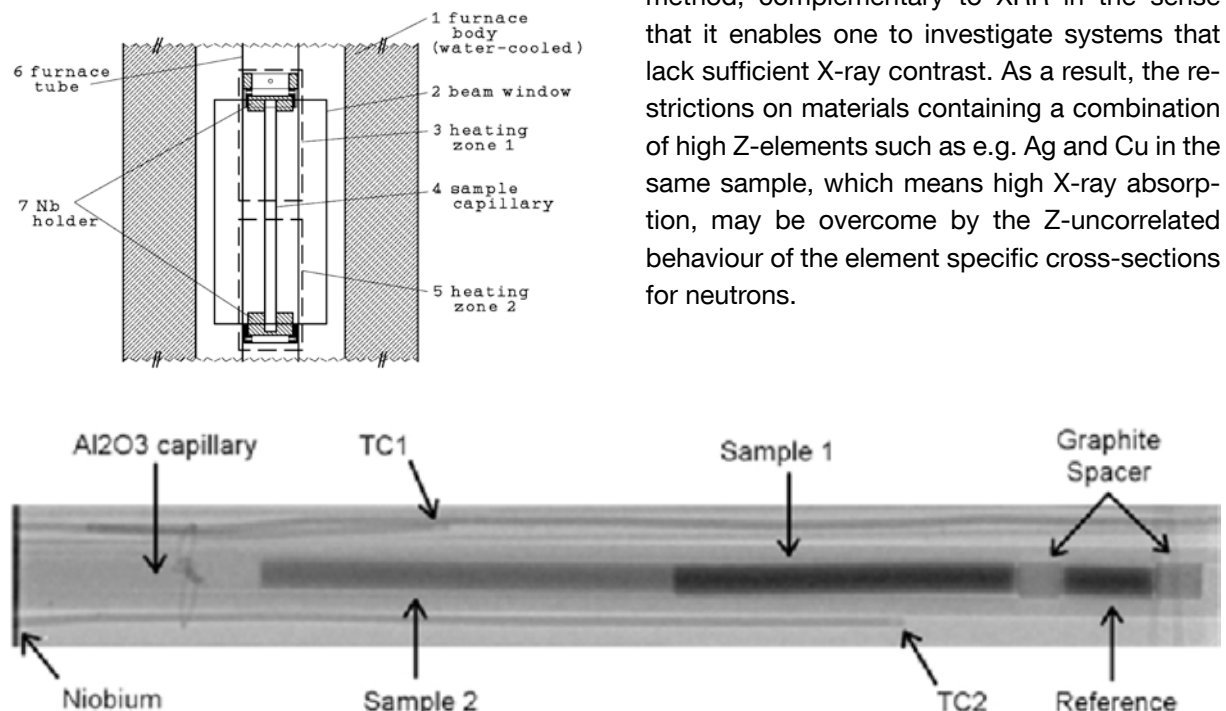
Figure 1: Top: Schematic diagram of Al 2 O 3 tube furnace. Bottom: Radiographic image of furnace including the Ag-Al-Cu diffusion couple. The darker vertical wires close to the diffusion couple represent the thermocouples.
